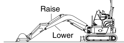
Boom cylinder
